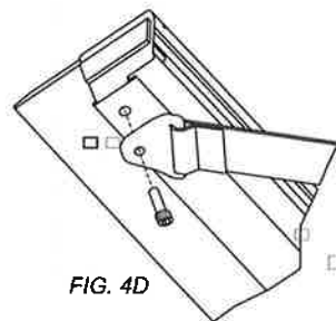
Plastic Shims
